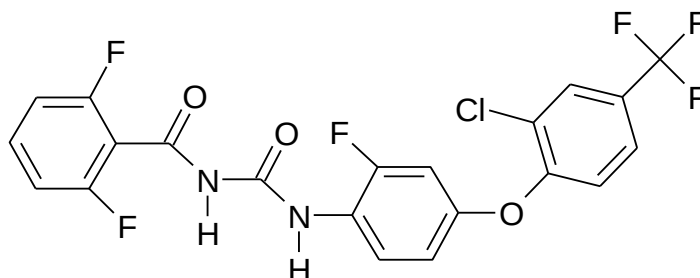
Flufenoxuron
